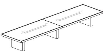
CX1635W+ELE L362 P122 H75 CX1647W+ELE L474 P122 H75
